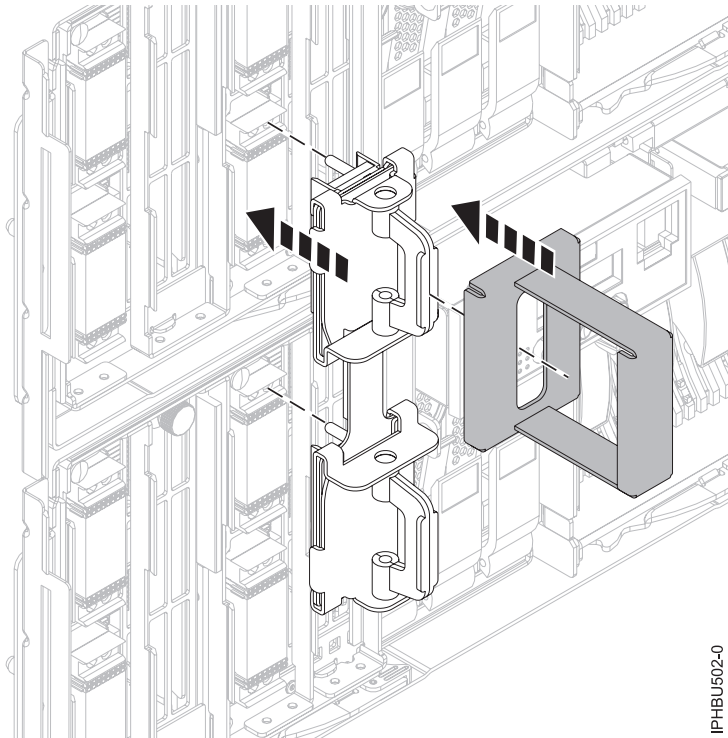
Figure 169. Using the SMP cable tool
