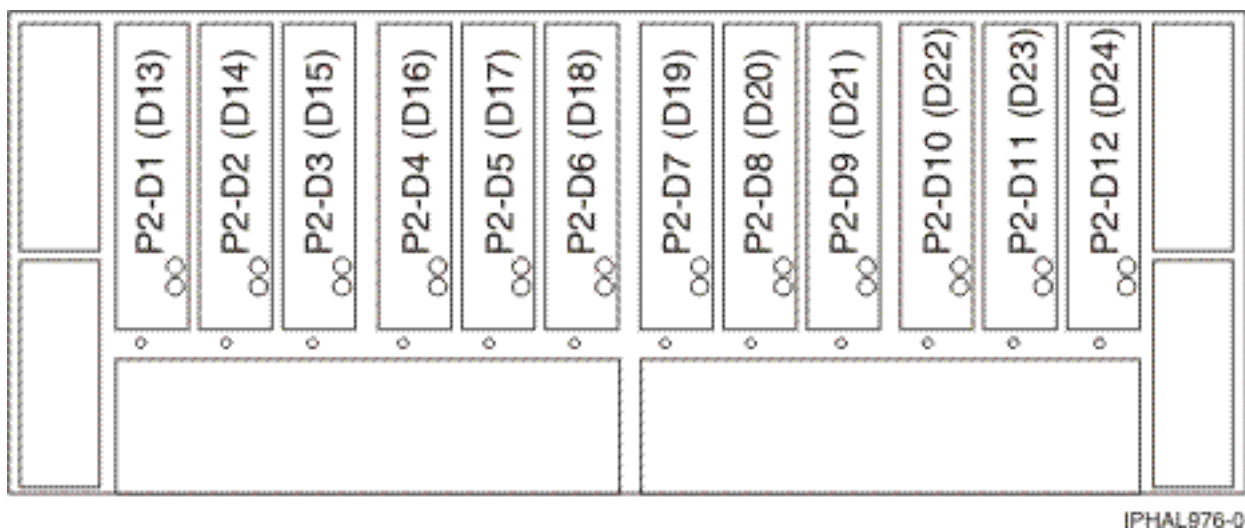
Figure 115. Back view of 5786, 5787, 7031-D24, and 7031-T24 SCSI disk-drive enclosures
