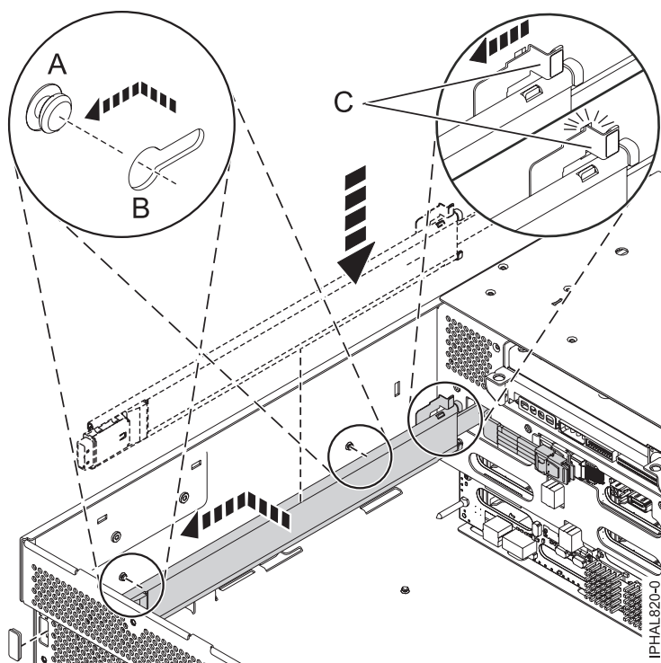
Figure 134. Placement of the SAS cable assembly
