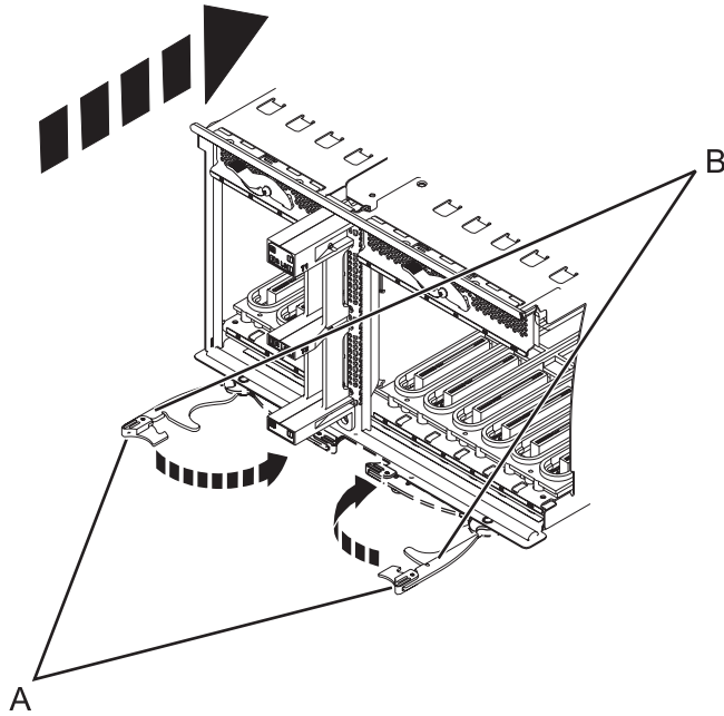
Figure 149. Install the I/O planar on a rack mounted model
