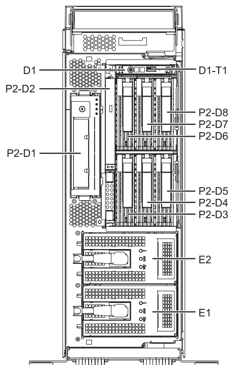
Figure 119. Disk drive locations for the SAS disk drives
