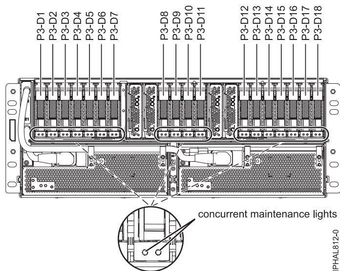
Figure 116. Disk drive locations
