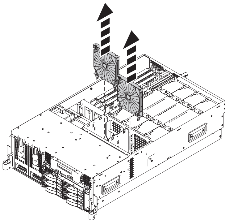
Figure 139. Removing the air baffles from the 8204-E8A or 9409-M50 fan cage
