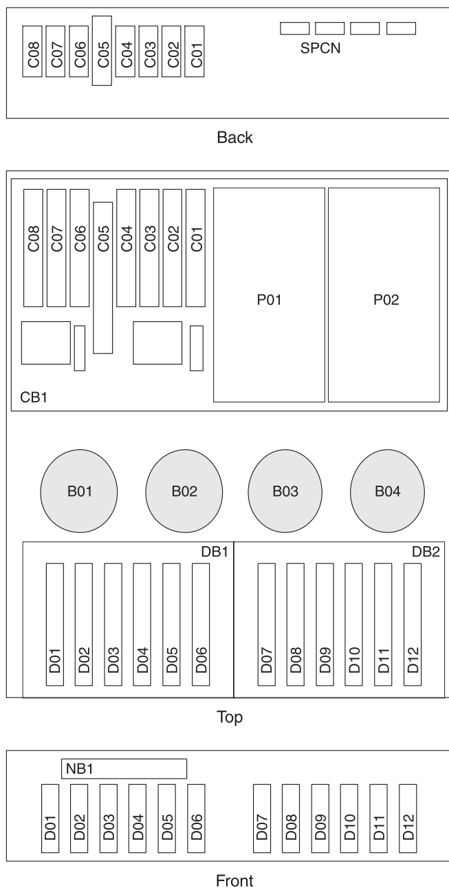
Figure 110. Model 0595 disk drive locations
