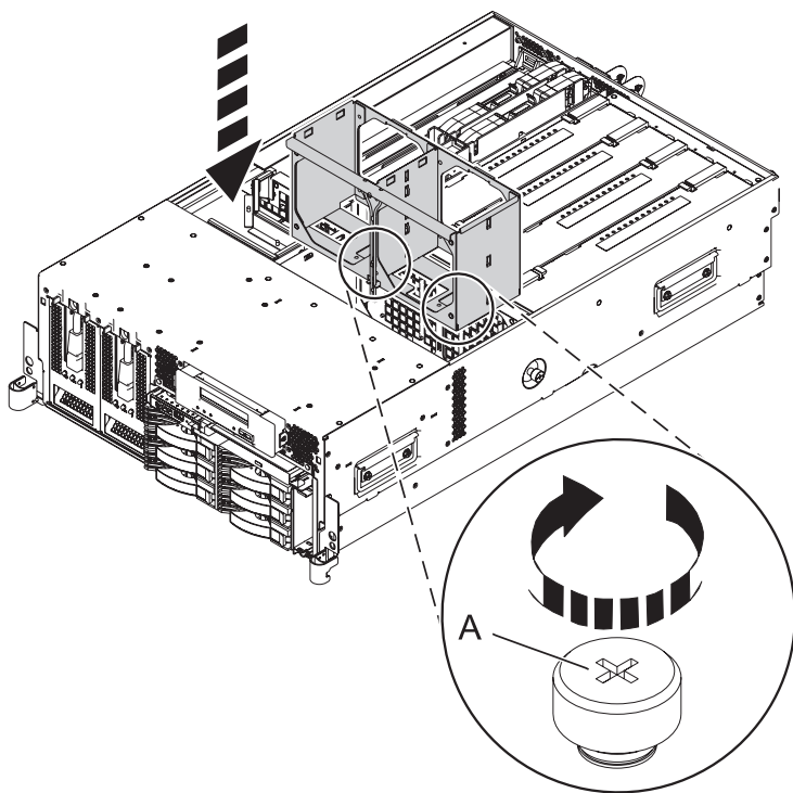
Figure 143. Installing the fan cage in the 8204-E8A or 9409-M50 system
