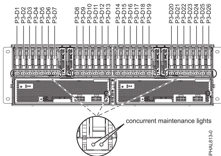
Figure 117. Disk drive locations
