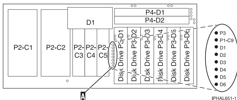
Figure 118. Model 9117-MMA/9406-MMA disk-drive concurrent maintenance lights
