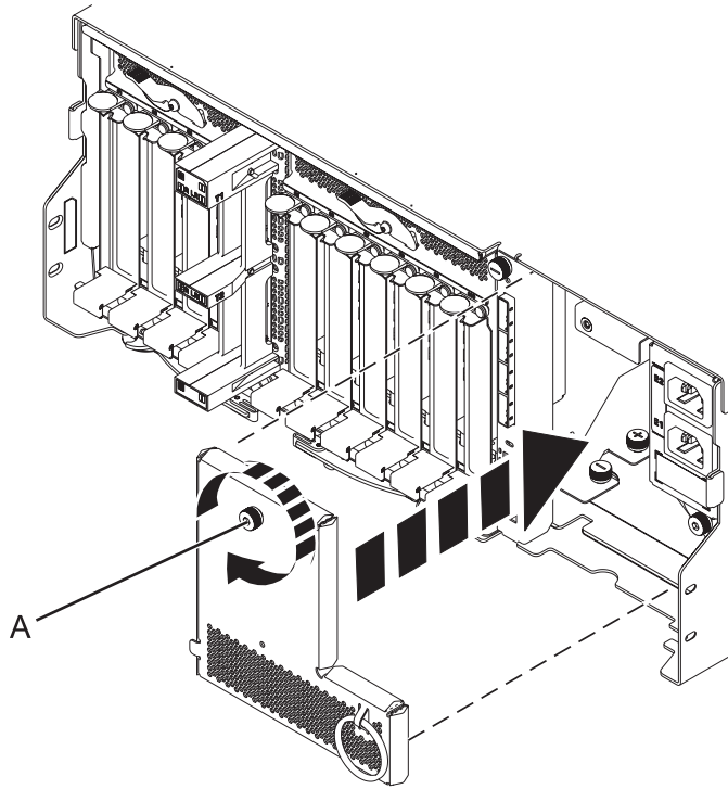
Figure 147. Installing the power cord plate
