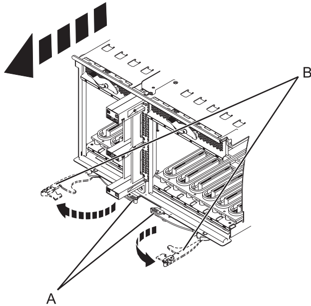
Figure 159. Removing the I/O planar
