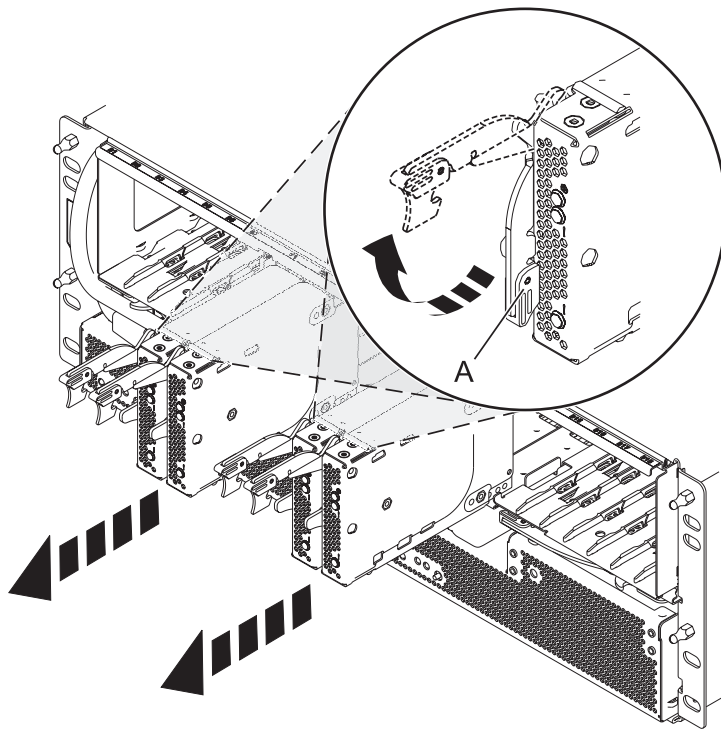
Figure 163. Removing the SAS expander card.
