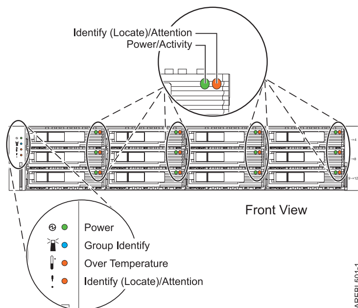
Figure 124. Front view of disk-drive enclosure concurrent maintenance lights for model 5886
