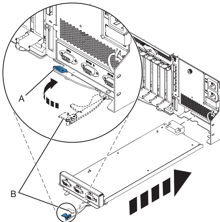
Figure 148. Replacing the enclosure management controller
