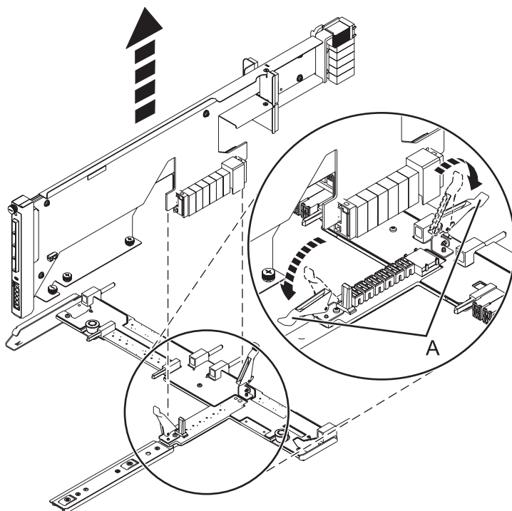
Figure 161. Removing the SAS conduit card from the midplane
