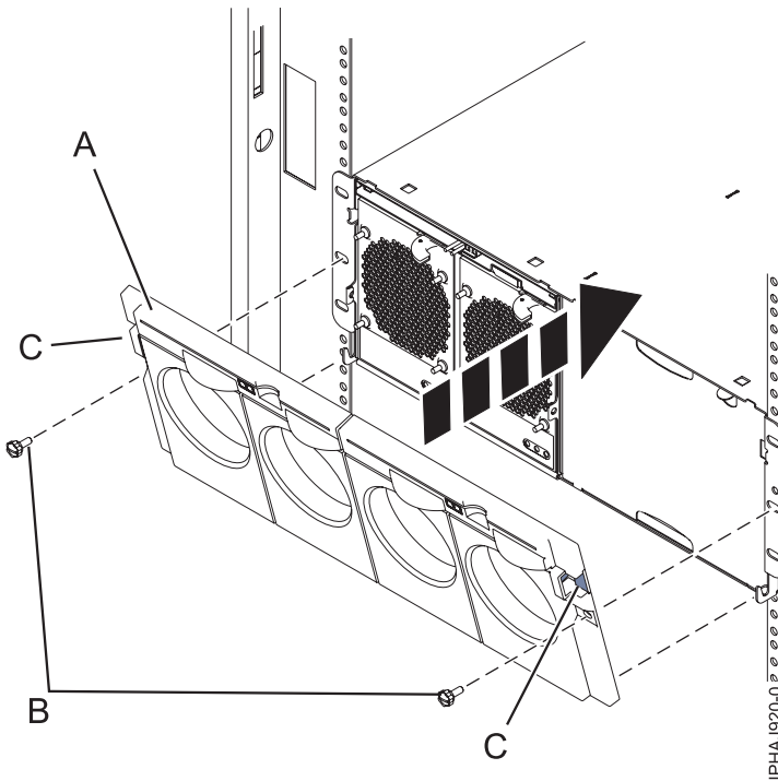
Figure 167. Front cover on a model 7314-G30 or 5796
