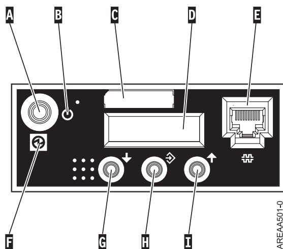
Figure 164. 570 control panel
