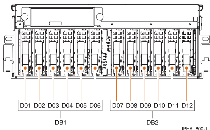
Figure 109. Disk drive locations for the 7311-D20 expansion unit
