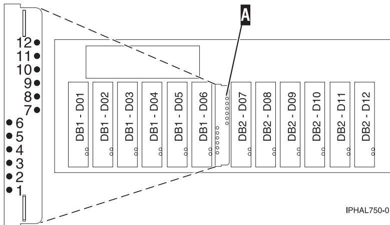
Figure 121. Model 7311-D20 disk-drive concurrent maintenance lights
