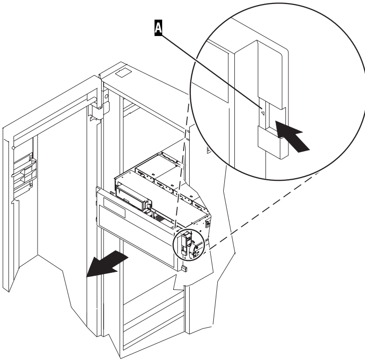
Figure 168. Removing the front cover
