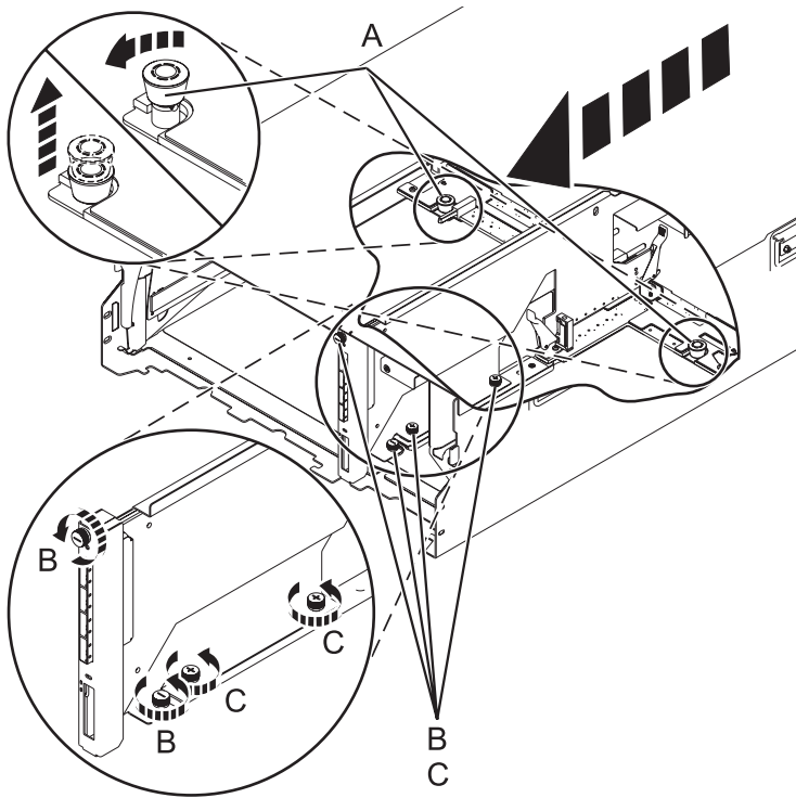
Figure 160. Removing the SAS conduit card and midplane
