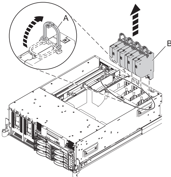
Figure 132. Removing the fans from the 8203-E4A, 8261-E4S, , 9407-M15, or 9408-M25 airflow cover
