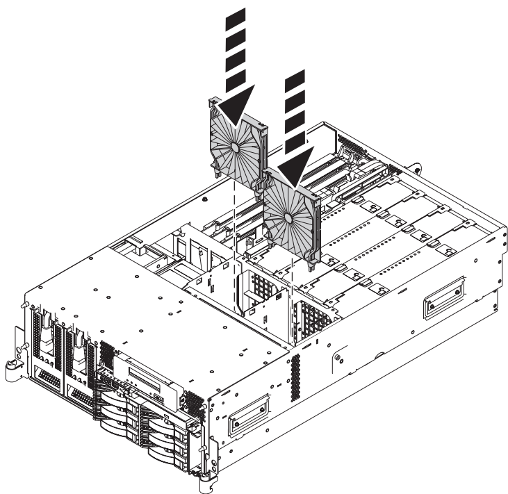
Figure 144. Installing the air baffles in the 8204-E8A or 9409-M50 fan cage
