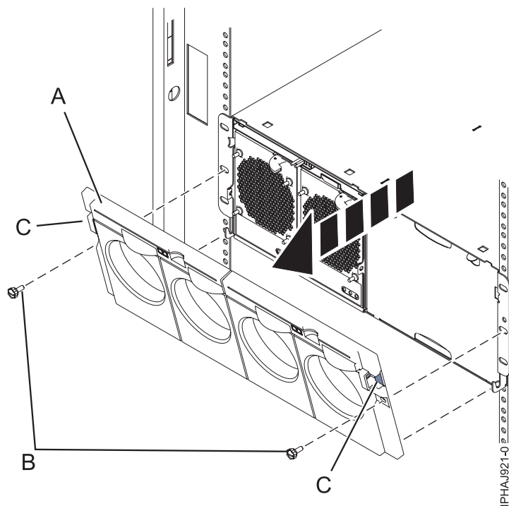
Figure 166. Remove the front cover for model 7314-G30 or 5796
