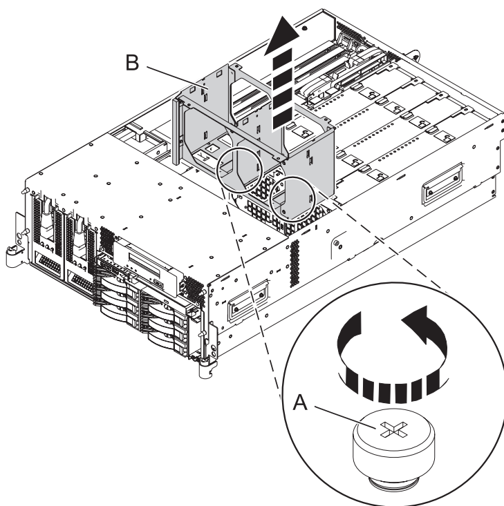
Figure 140. Removing the fan cage from the 8204-E8A or 9409-M50 system
