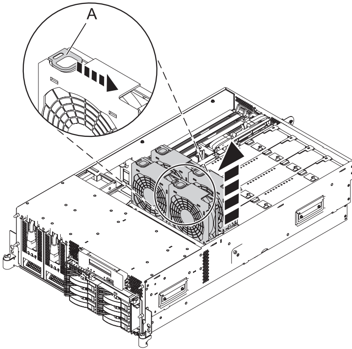
Figure 138. Removing the fan from the 8204-E8A or 9409-M50 fan cage
