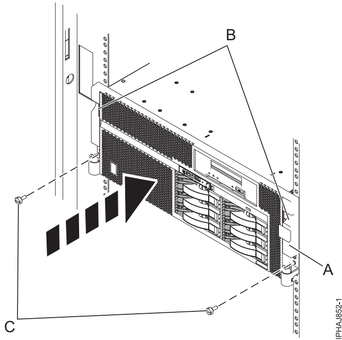
Figure 183. Pushing the system into the rack and attaching the thumbscrews
