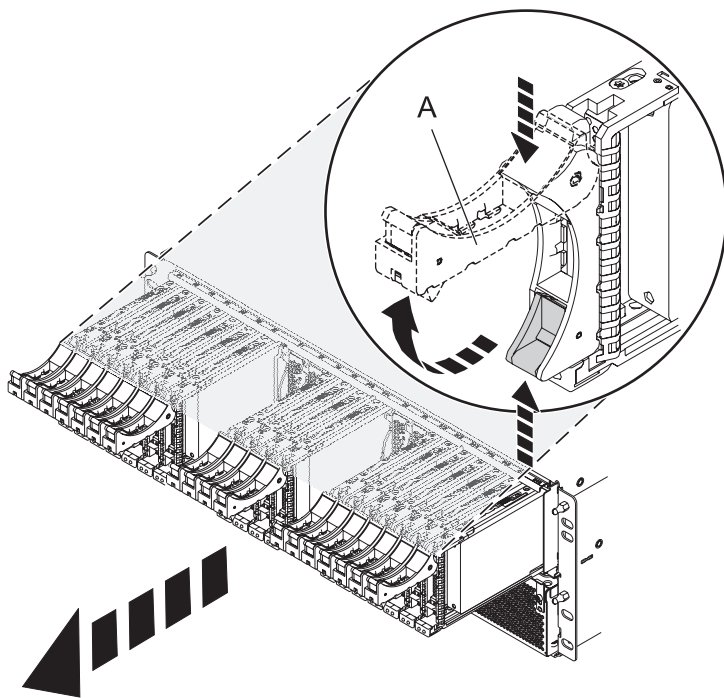
Figure 152. Removing the disk drives from the backplane
