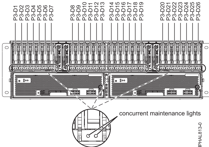
Figure 126. Disk drive locations
