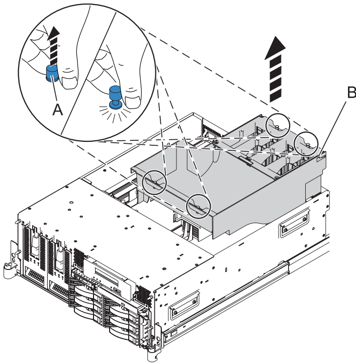
Figure 133. Removing the airflow cover from the 8203-E4A, 8261-E4S, , 9407-M15, or 9408-M25 system
