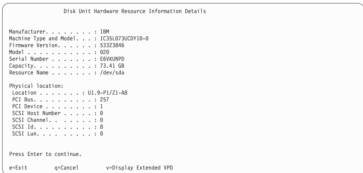
Figure 55. Disk Unit Hardware Resource Information Details display
