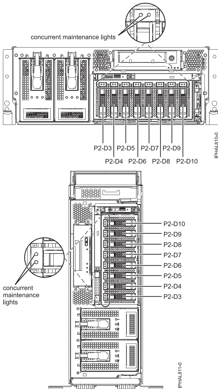
Figure 112. Disk drive locations for small form factor disk drives
