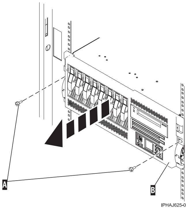
Figure 180. Removing the thumbscrews from the system and rack
