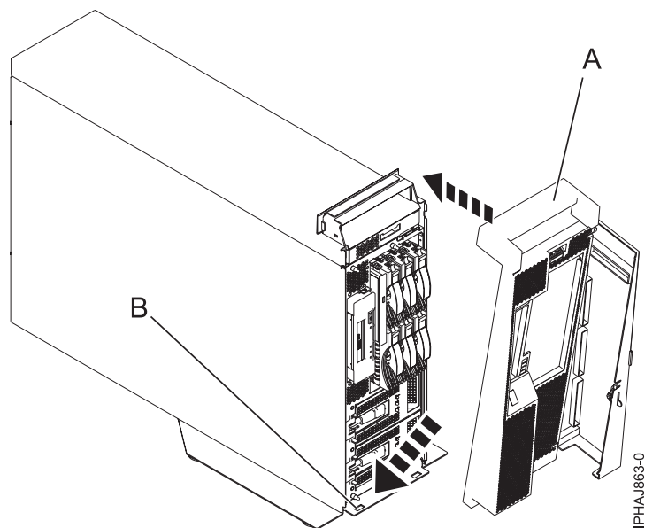
Figure 177. Replacing the cover on the model
