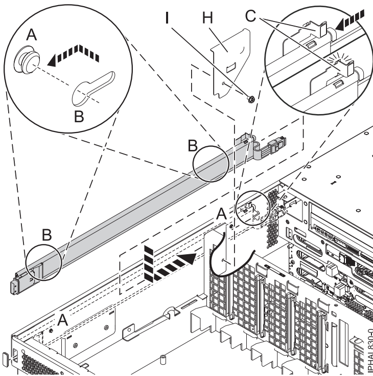
Figure 141. Attaching the SAS cable
