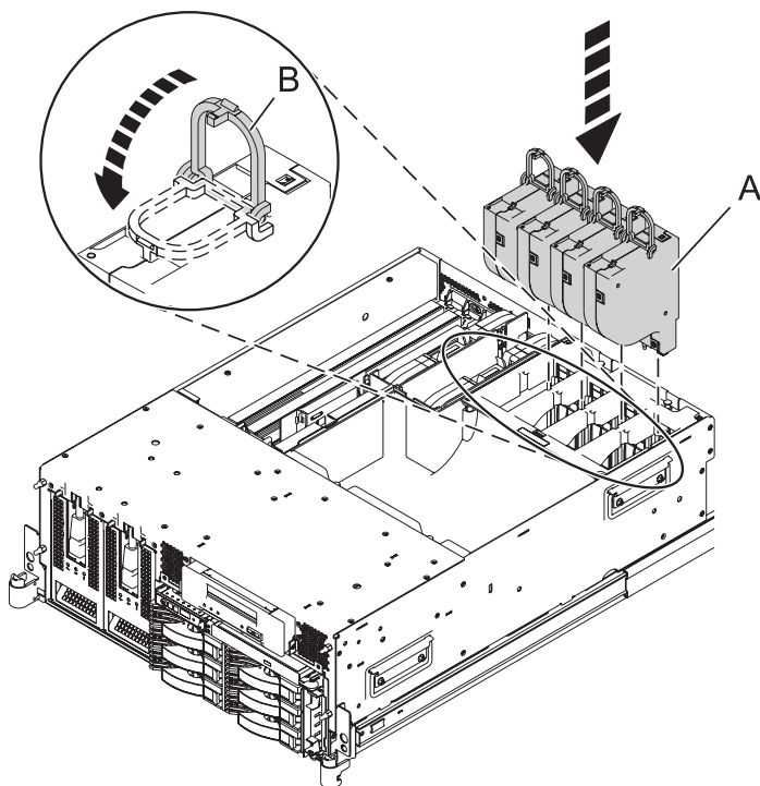
Figure 137. Installing the fans in the 8203-E4A, 8261-E4S, 9407-M15, or 9408-M25 airflow cover
