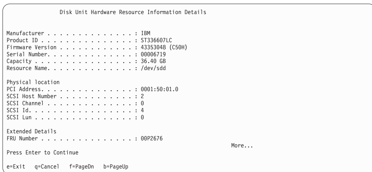
Figure 71. Example Disk Hardware Resource Information Details display
