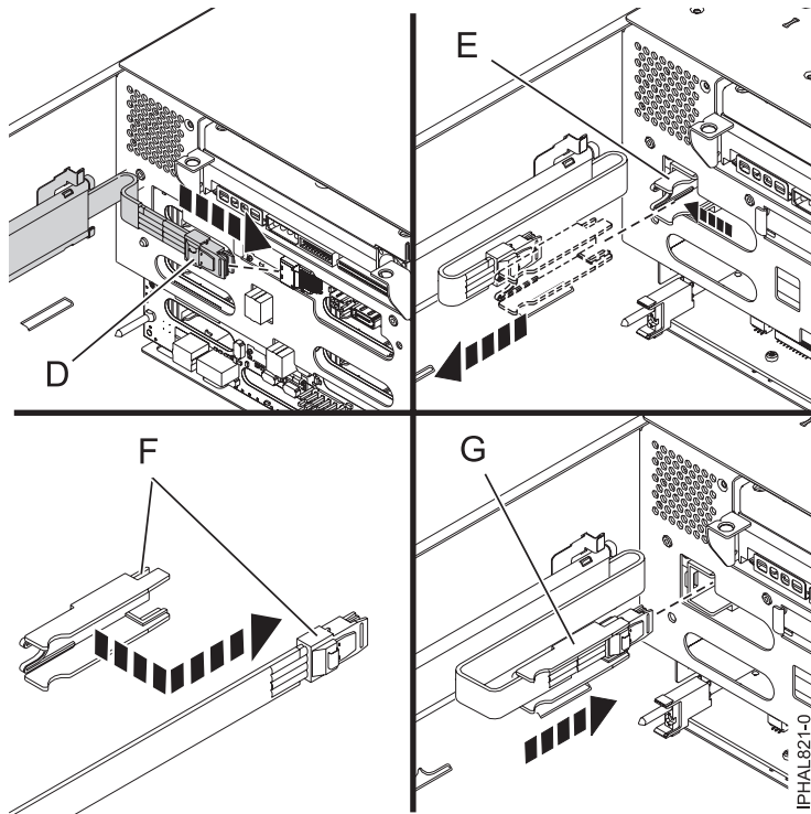
Figure 142. SAS cable connections
