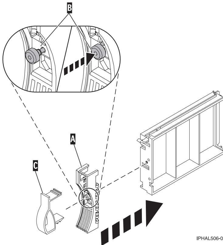
Figure 106. Attaching a bezel to a disk-drive filler
