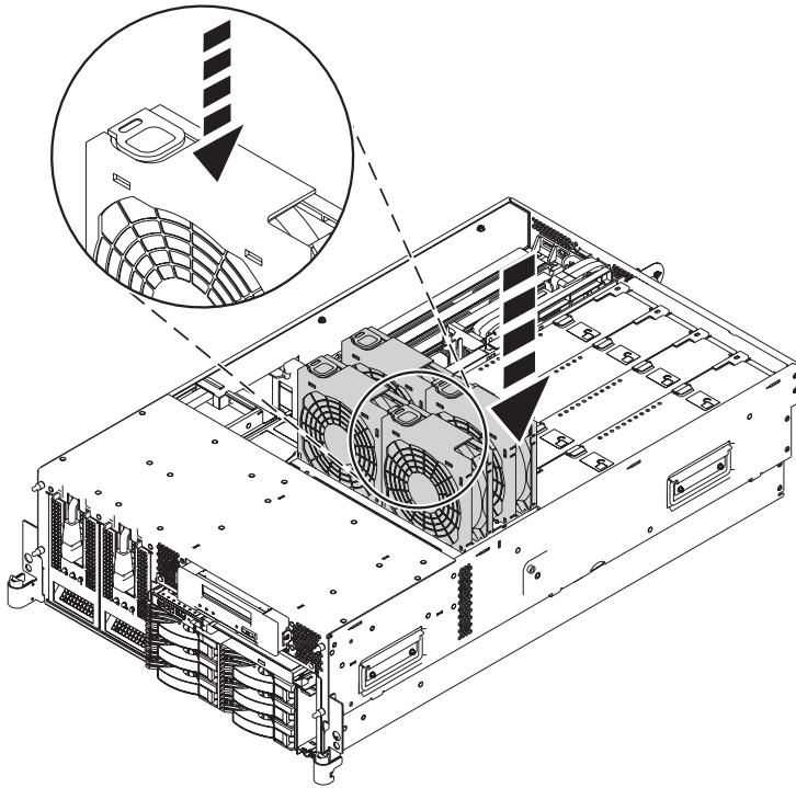
Figure 145. Installing the fans in the 8204-E8A or 9409-M50 fan cage
