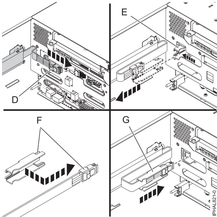
Figure 135. SAS cable connections
