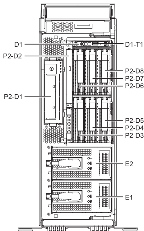
Figure 111. Disk drive locations for the SAS disk drives
