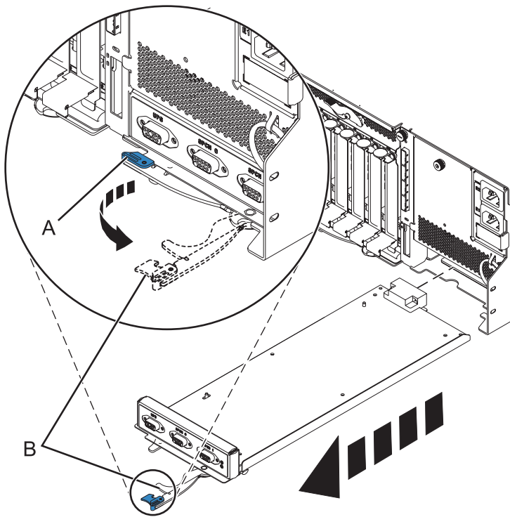
Figure 157. Remove the enclosure management controller
