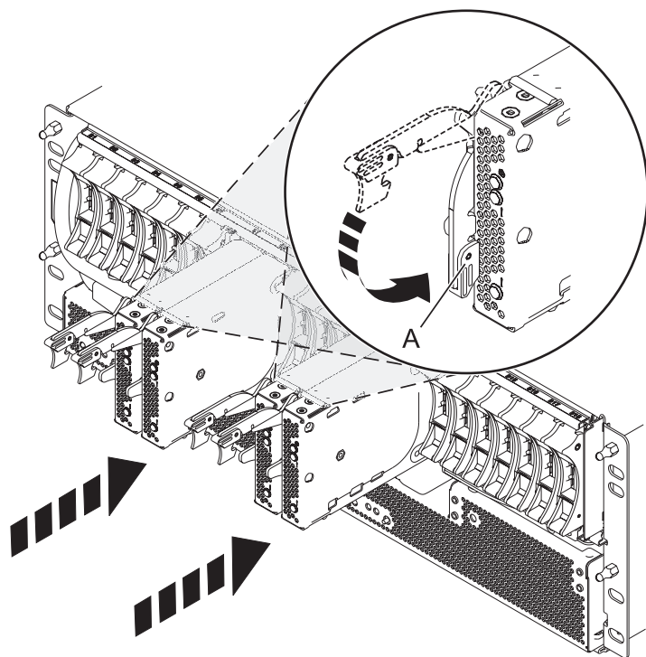
Figure 162. Installing the SAS expander card
