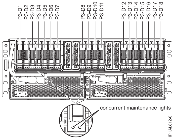
Figure 125. Disk drive locations
