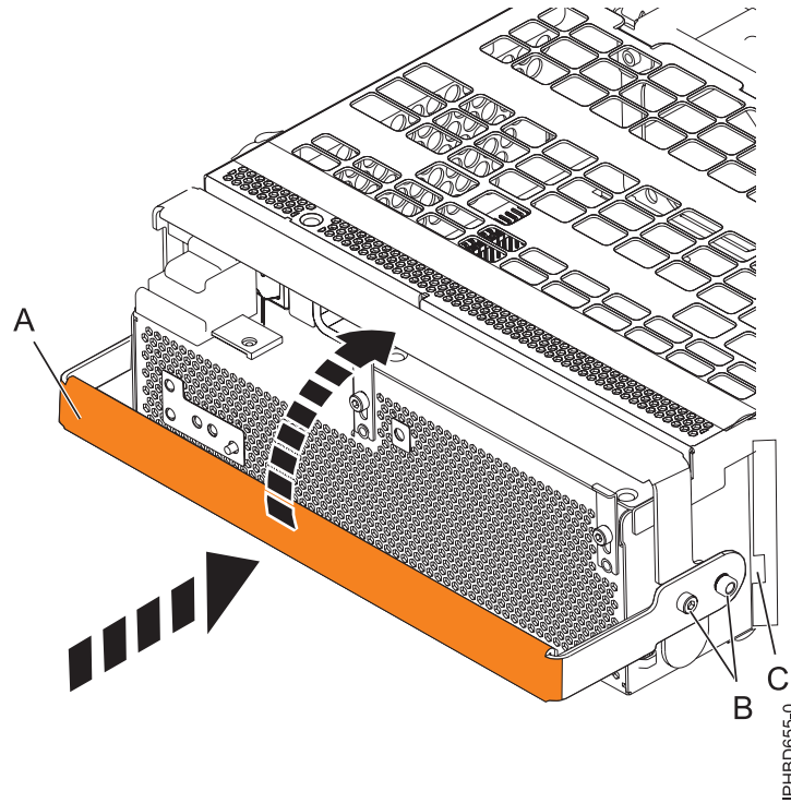
Figure 150. Replacing a power supply
